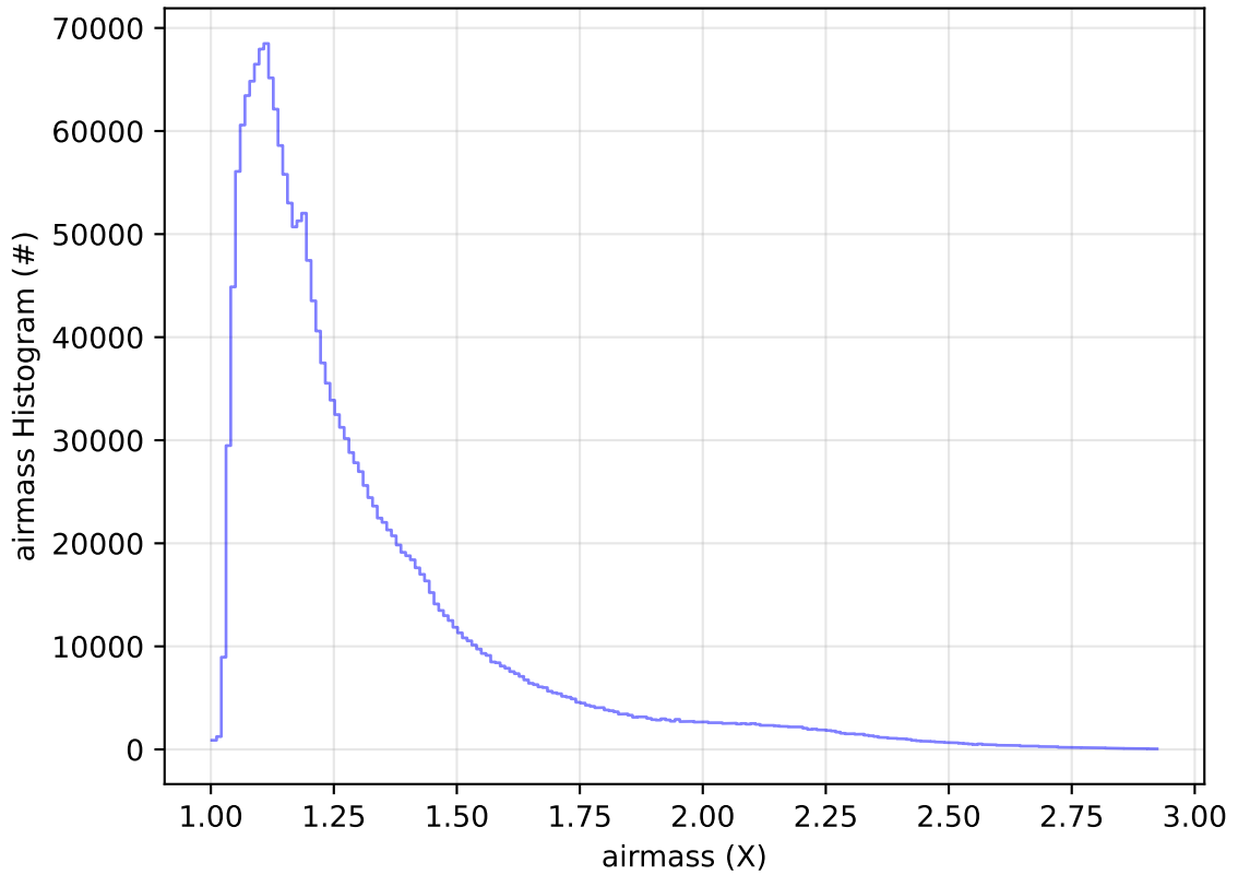
roll_uniform_early_half_accordion1_mjdp0_v3.4_10yrs All sky all bands: airmass Histogram
