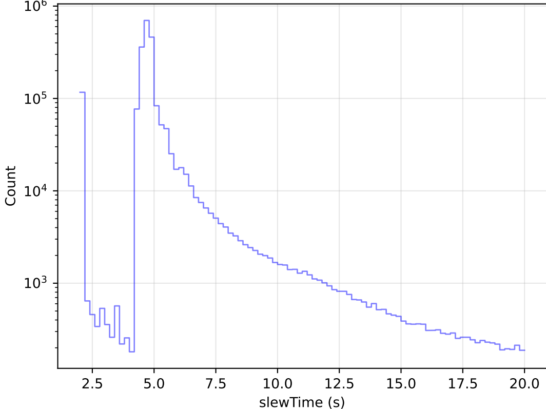
roll_uniform_early_half_accordion1_mjdp0_v3.4_10yrs All visits: Zoom Slew Time Histogram
