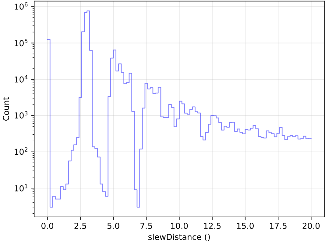
roll_uniform_early_half_accordion1_mjdp0_v3.4_10yrs All visits: Zoom Slew Distance Histogram
