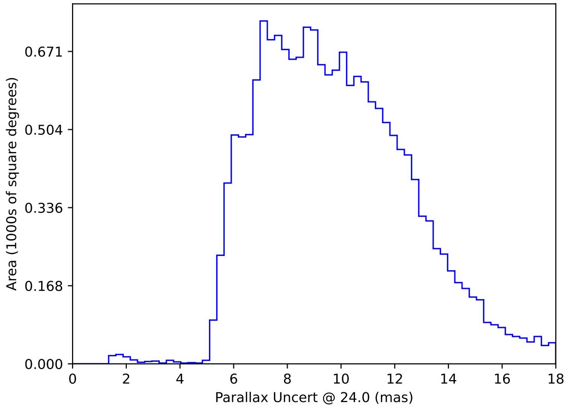
roll_uniform_early_half_accordion1_mjdp0_v3.4_10yrs WFD: Parallax Uncert @ 24.0
