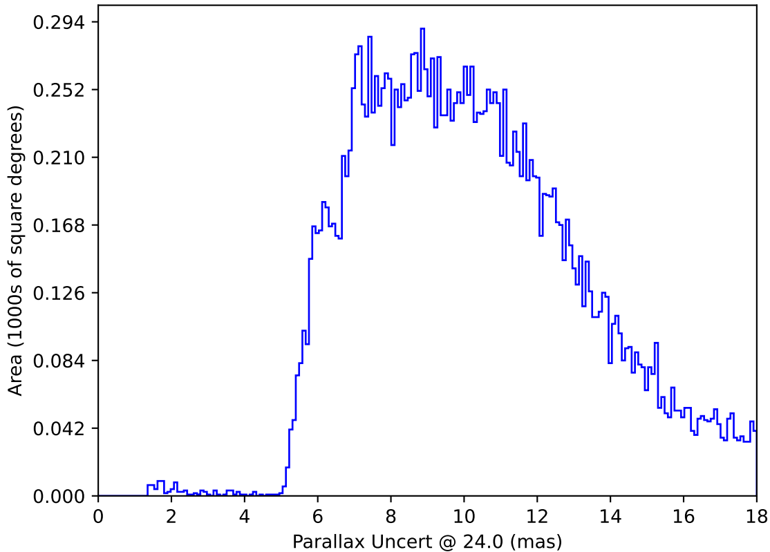
roll_uniform_early_half_accordion1_mjdp0_v3.4_10yrs All sky: Parallax Uncert @ 24.0
