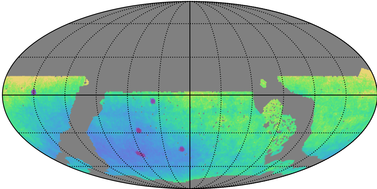
roll_uniform_early_half_accordion1_mjdp0_v3.4_10yrs WFD y band only: Parallax Uncert @ 21.3
