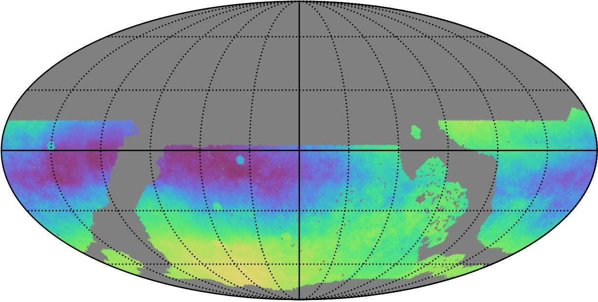
roll_uniform_early_half_accordion1_mjdp0_v3.4_10yrs WFD: Parallax-DCR degeneracy @ 24.0
