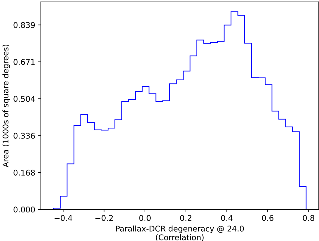
roll_uniform_early_half_accordion1_mjdp0_v3.4_10yrs WFD: Parallax-DCR degeneracy @ 24.0
