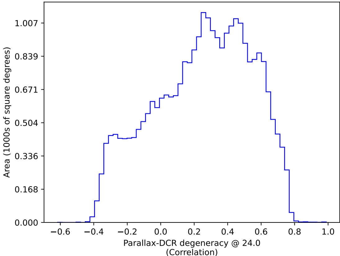
roll_uniform_early_half_accordion1_mjdp0_v3.4_10yrs All sky: Parallax-DCR degeneracy @ 24.0
