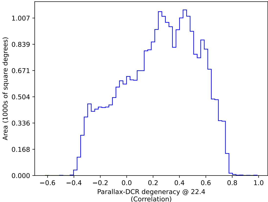
roll_uniform_early_half_accordion1_mjdp0_v3.4_10yrs All sky: Parallax-DCR degeneracy @ 22.4
