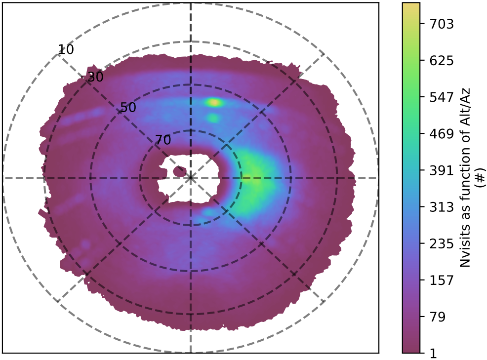
roll_uniform_early_half_accordion1_mjdp0_v3.4_10yrs u band: Nvisits as function of Alt/Az
