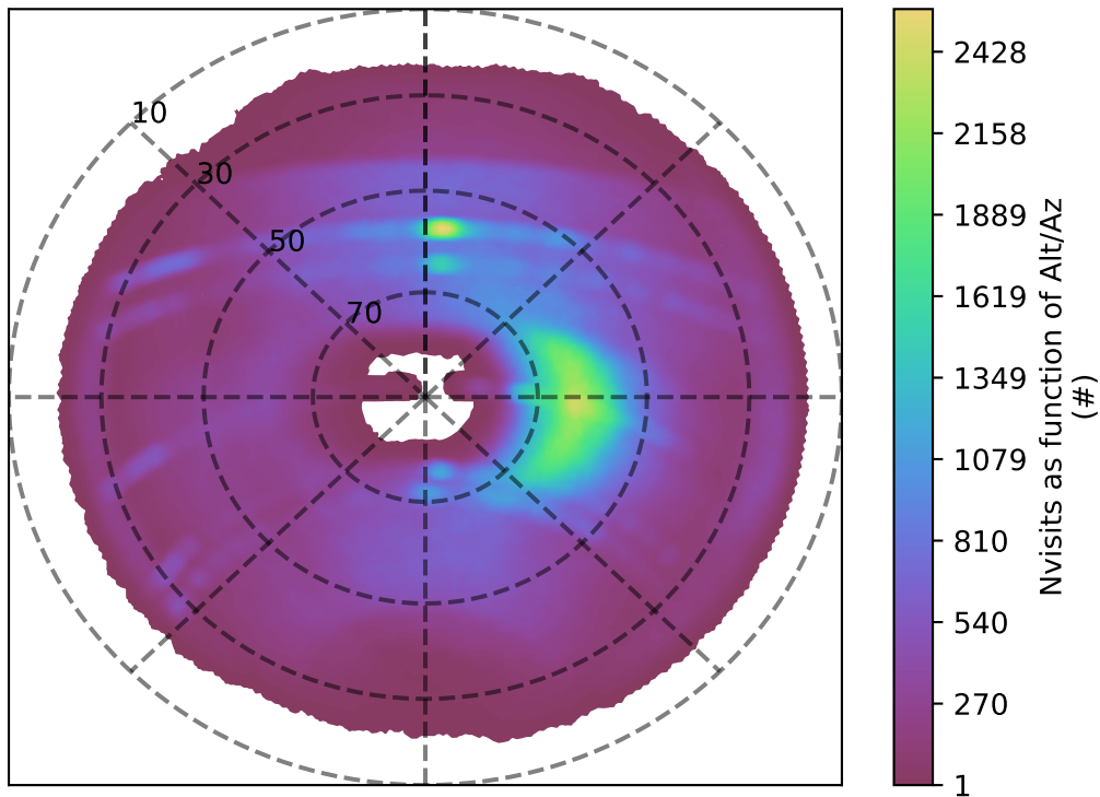
roll_uniform_early_half_accordion1_mjdp0_v3.4_10yrs i band: Nvisits as function of Alt/Az
