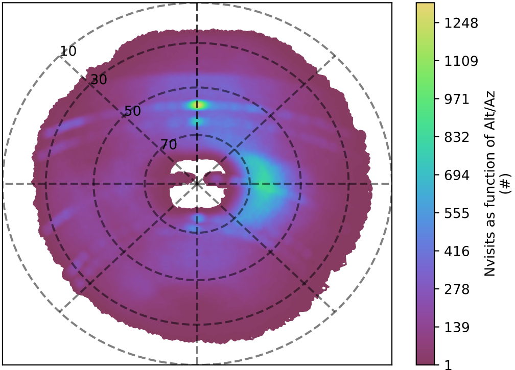
roll_uniform_early_half_accordion1_mjdp0_v3.4_10yrs g band: Nvisits as function of Alt/Az
