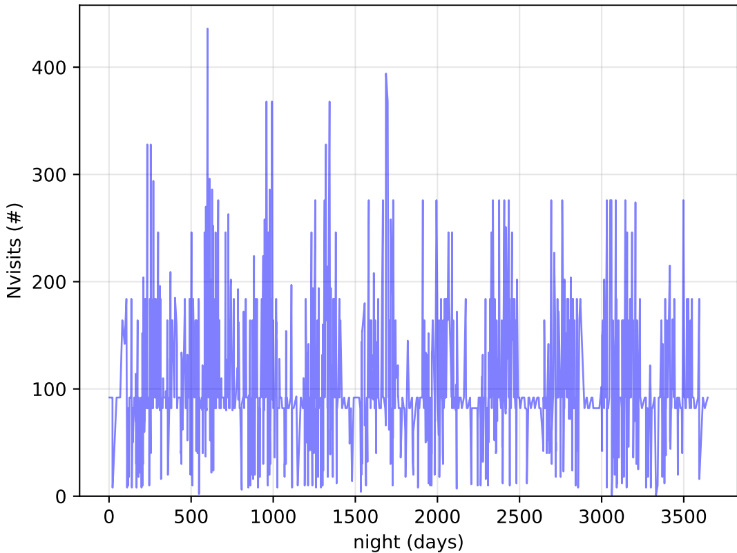
roll_uniform_early_half_accordion1_mjdp0_v3.4_10yrs DDF: Nvisits
