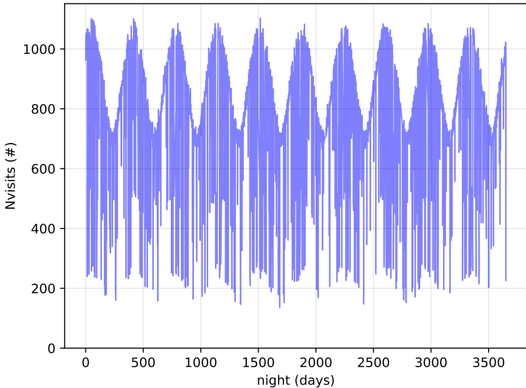
roll_uniform_early_half_accordion1_mjdp0_v3.4_10yrs All visits: Nvisits
