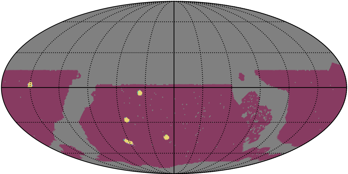
roll_uniform_early_half_accordion1_mjdp0_v3.4_10yrs WFD: NumberOfQuickRevisits
