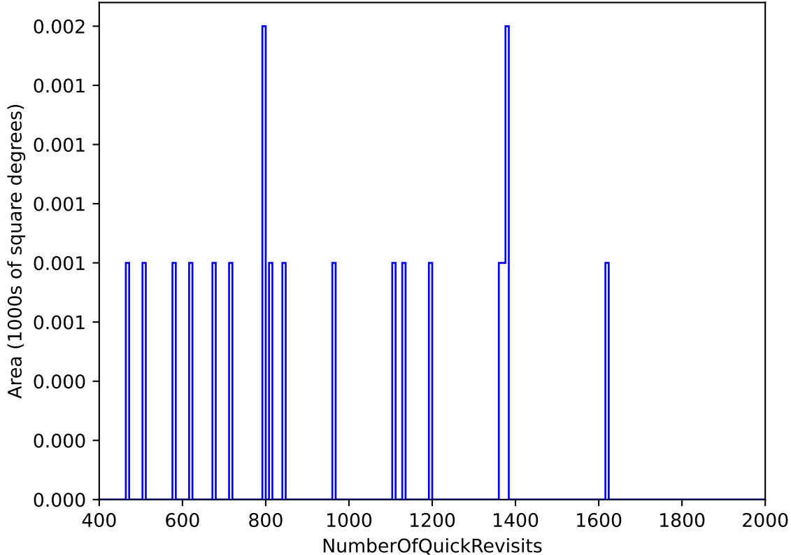
roll_uniform_early_half_accordion1_mjdp0_v3.4_10yrs WFD: NumberOfQuickRevisits
