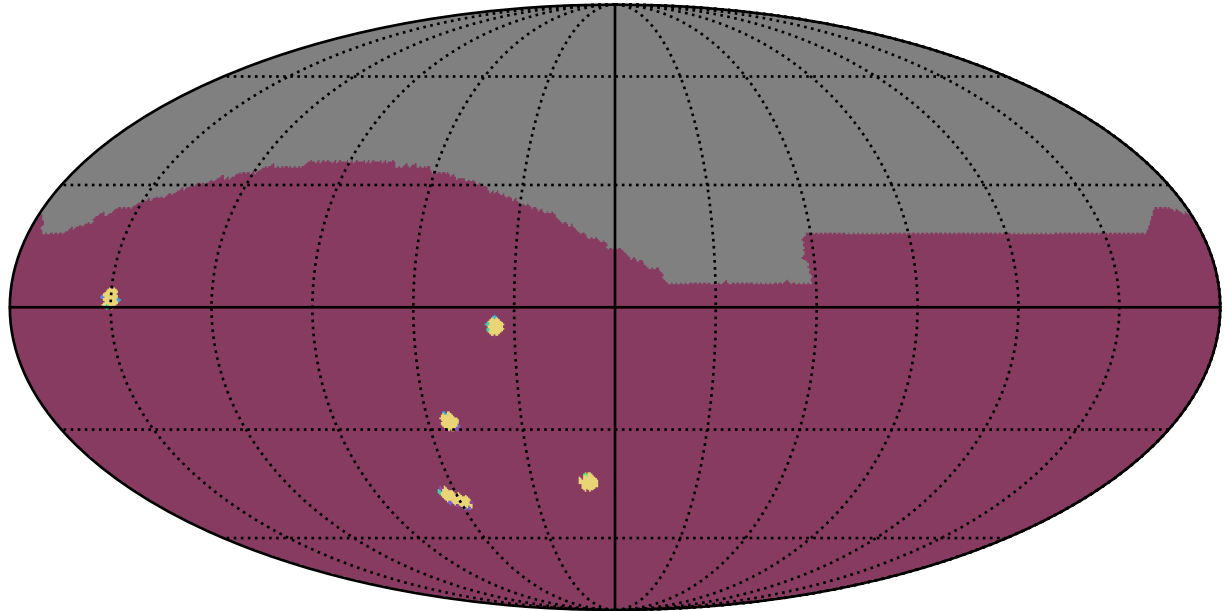
roll_uniform_early_half_accordion1_mjdp0_v3.4_10yrs All sky: NumberOfQuickRevisits
