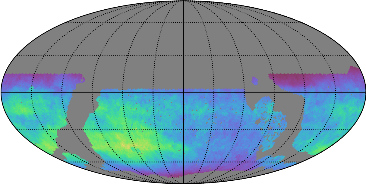
roll_uniform_early_half_accordion1_mjdp0_v3.4_10yrs WFD z band: Normalized Teff
