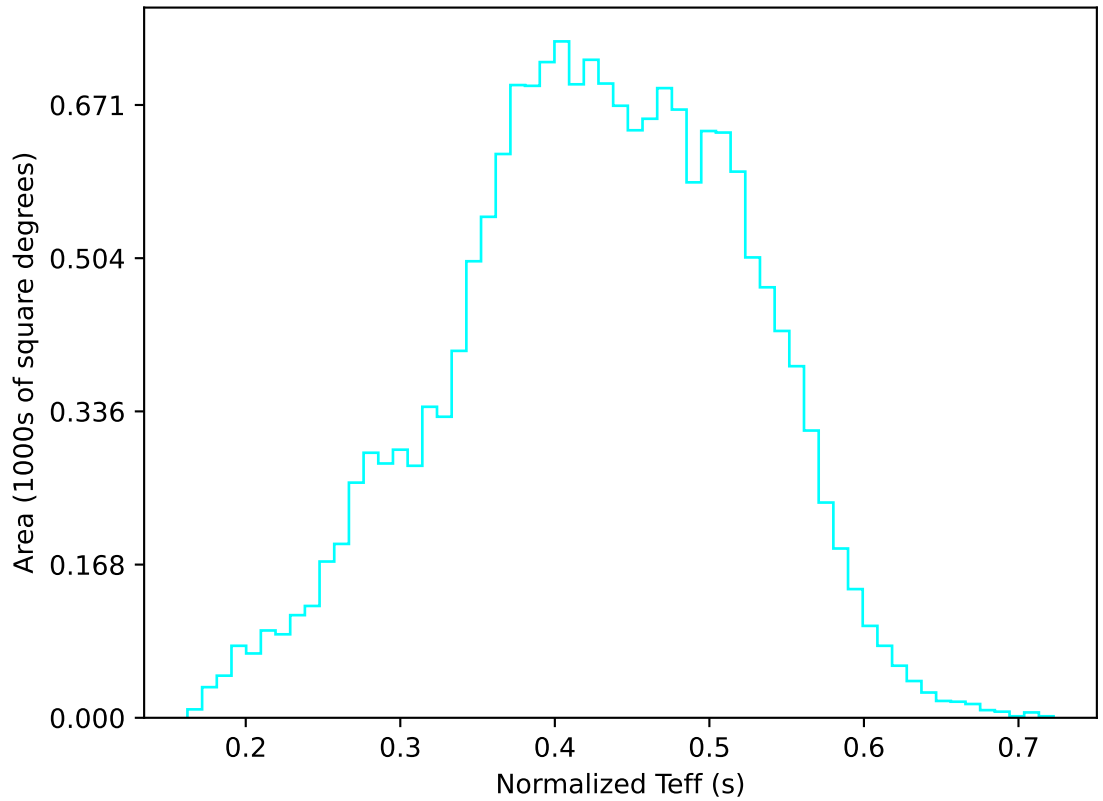
roll_uniform_early_half_accordion1_mjdp0_v3.4_10yrs WFD u band: Normalized Teff
