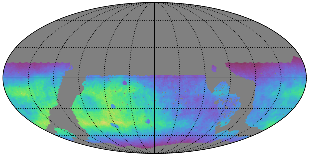
roll_uniform_early_half_accordion1_mjdp0_v3.4_10yrs WFD r band: Normalized Teff
