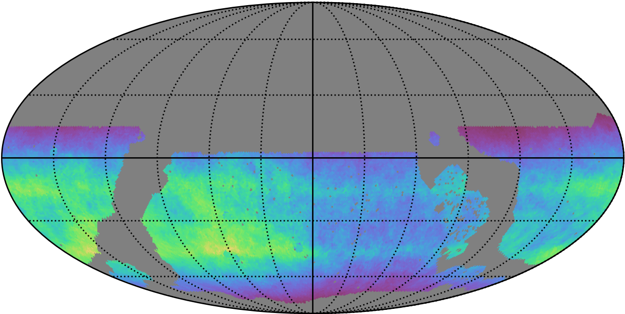
roll_uniform_early_half_accordion1_mjdp0_v3.4_10yrs WFD i band: Normalized Teff
