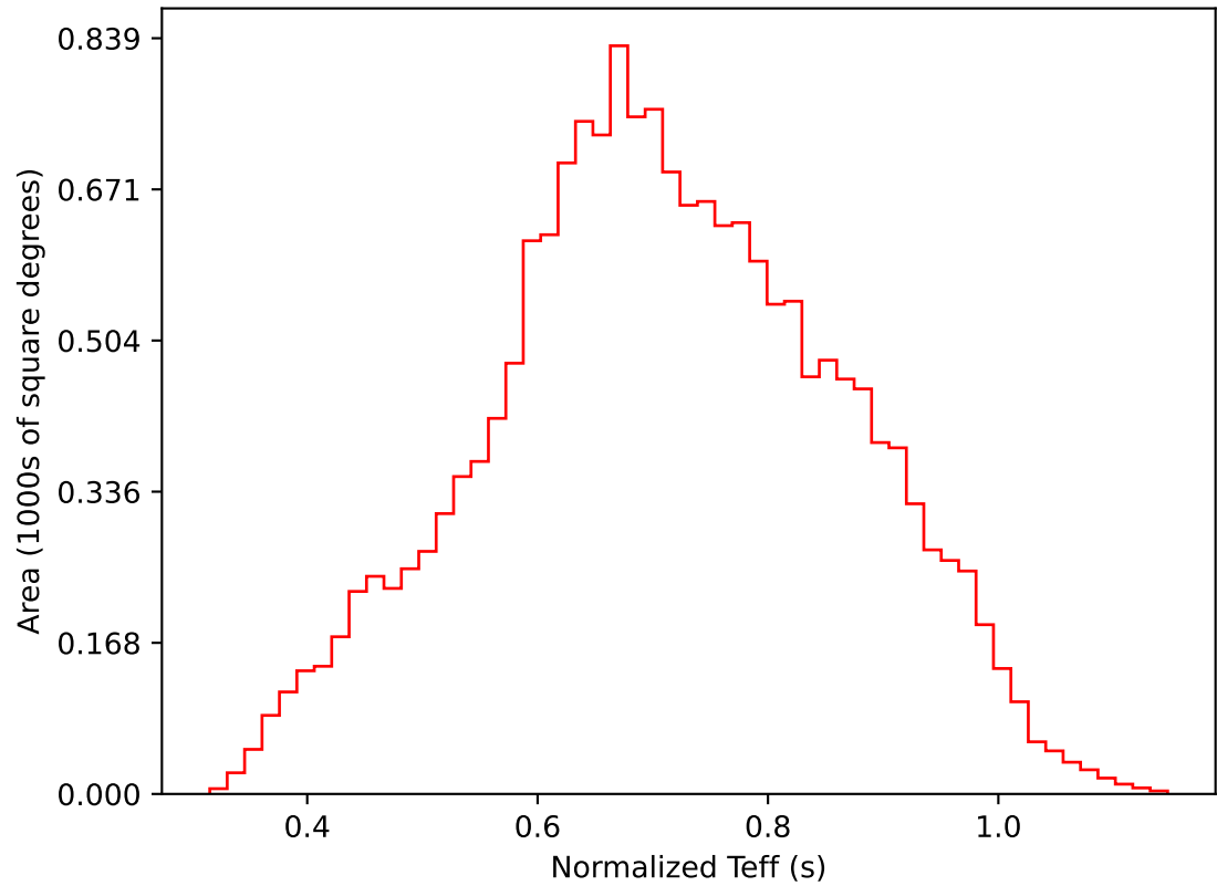
roll_uniform_early_half_accordion1_mjdp0_v3.4_10yrs WFD i band: Normalized Teff
