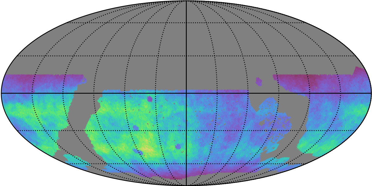
roll_uniform_early_half_accordion1_mjdp0_v3.4_10yrs WFD g band: Normalized Teff
