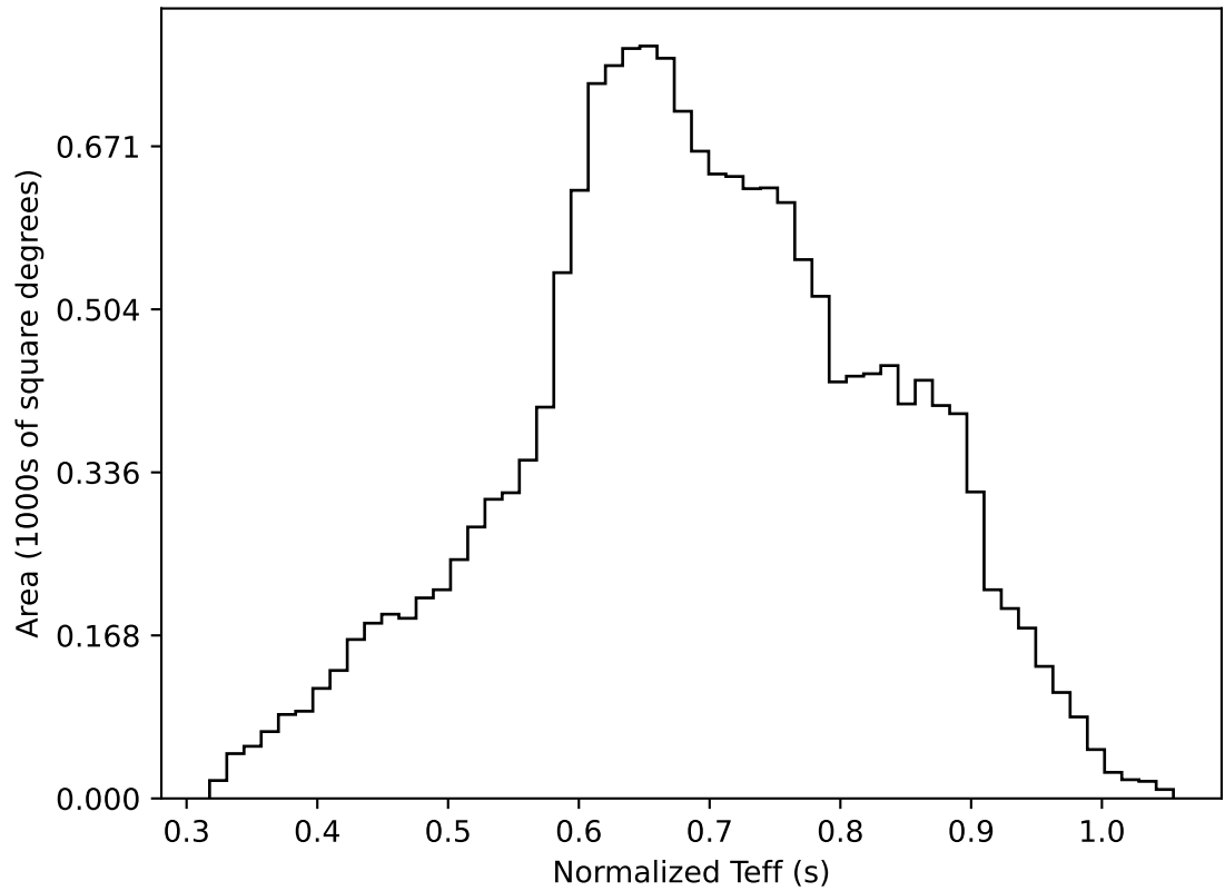
roll_uniform_early_half_accordion1_mjdp0_v3.4_10yrs WFD all bands: Normalized Teff
