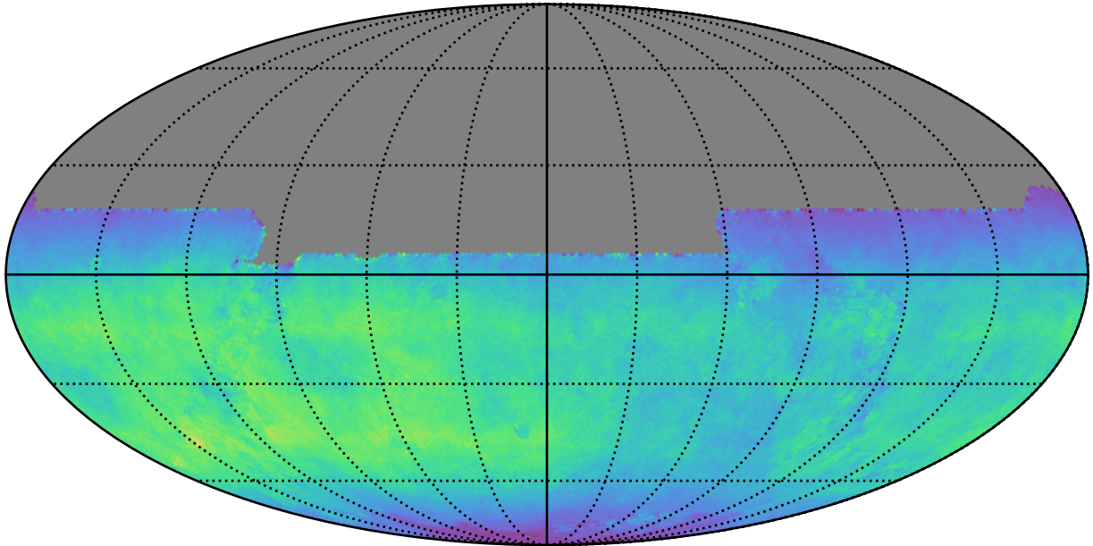
roll_uniform_early_half_accordion1_mjdp0_v3.4_10yrs All sky y band: Normalized Teff
