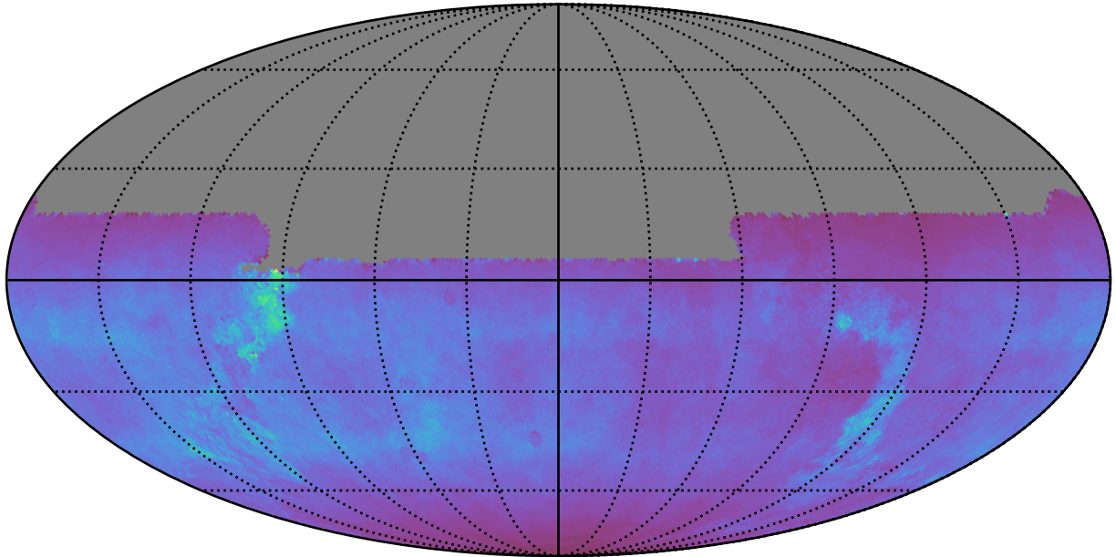
roll_uniform_early_half_accordion1_mjdp0_v3.4_10yrs All sky u band: Normalized Teff
