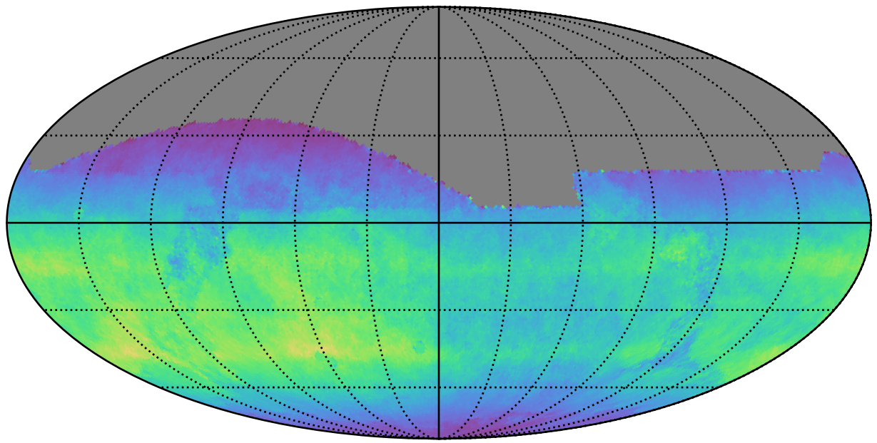
roll_uniform_early_half_accordion1_mjdp0_v3.4_10yrs All sky i band: Normalized Teff
