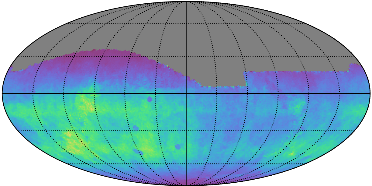
roll_uniform_early_half_accordion1_mjdp0_v3.4_10yrs All sky g band: Normalized Teff
