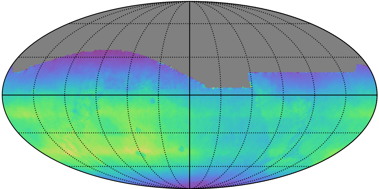
roll_uniform_early_half_accordion1_mjdp0_v3.4_10yrs All sky all bands: Normalized Teff
