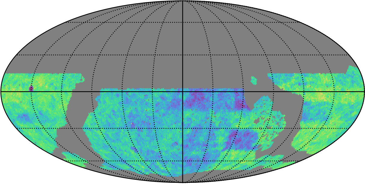
roll_uniform_early_half_accordion1_mjdp0_v3.4_10yrs WFD: Normalized Proper Motion Uncert @ 24.0
