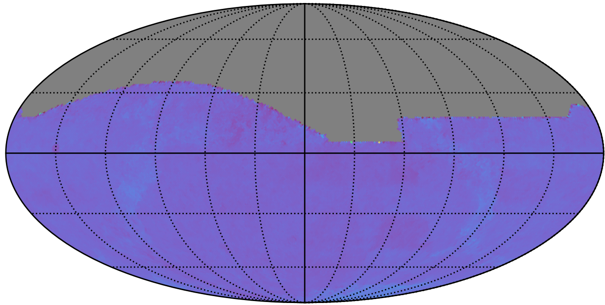
roll_uniform_early_half_accordion1_mjdp0_v3.4_10yrs All sky: Normalized Proper Motion Uncert @ 24.0
