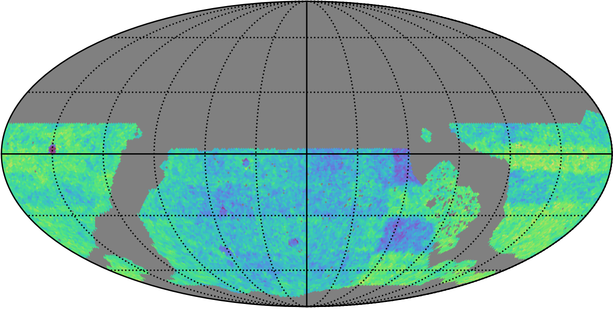
roll_uniform_early_half_accordion1_mjdp0_v3.4_10yrs WFD: Normalized Proper Motion Uncert @ 20.5
