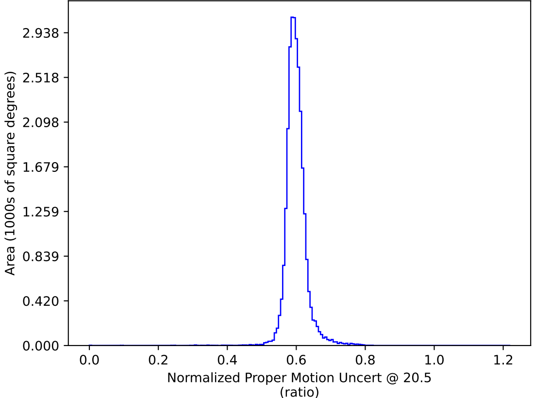
roll_uniform_early_half_accordion1_mjdp0_v3.4_10yrs All sky: Normalized Proper Motion Uncert @ 20.5
