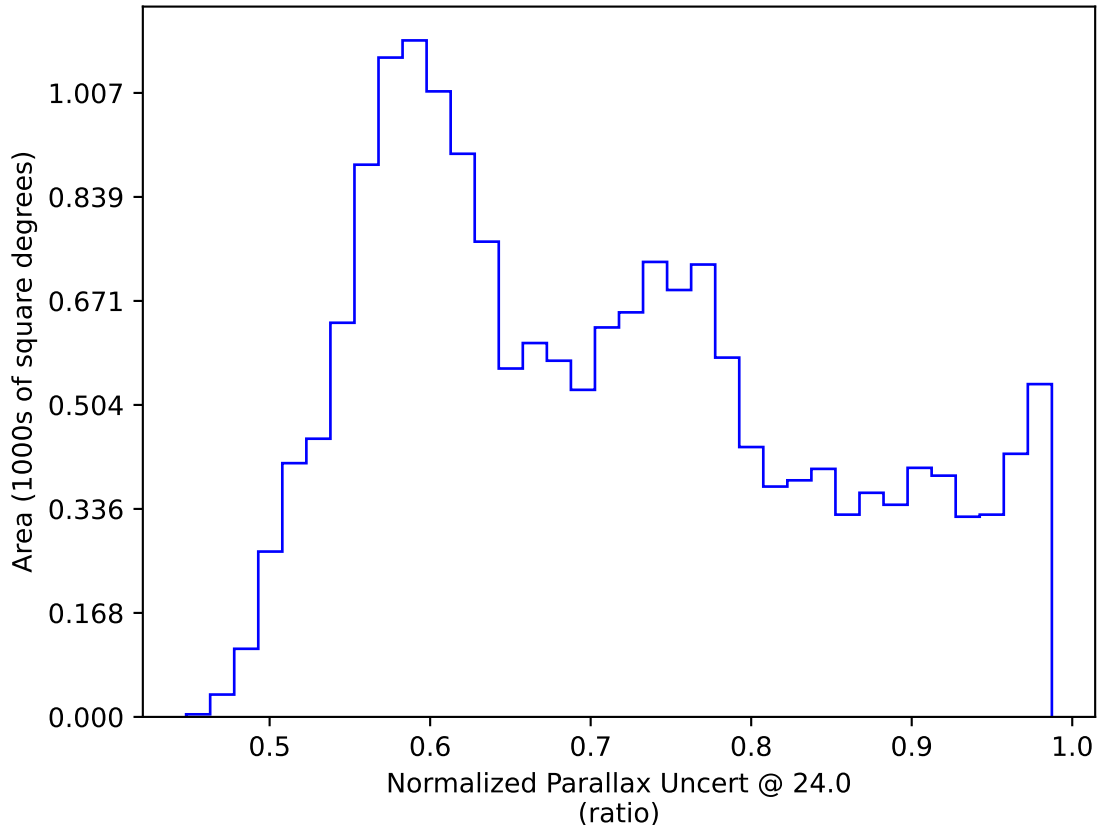
roll_uniform_early_half_accordion1_mjdp0_v3.4_10yrs WFD: Normalized Parallax Uncert @ 24.0
