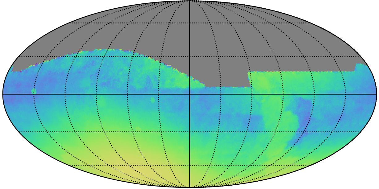
roll_uniform_early_half_accordion1_mjdp0_v3.4_10yrs All sky: Normalized Parallax Uncert @ 24.0
