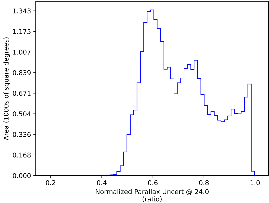
roll_uniform_early_half_accordion1_mjdp0_v3.4_10yrs All sky: Normalized Parallax Uncert @ 24.0
