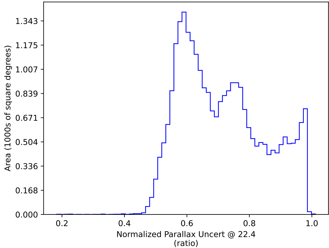
roll_uniform_early_half_accordion1_mjdp0_v3.4_10yrs All sky: Normalized Parallax Uncert @ 22.4
