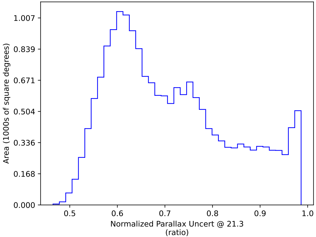
roll_uniform_early_half_accordion1_mjdp0_v3.4_10yrs WFD y band only: Normalized Parallax Uncert @ 21.3
