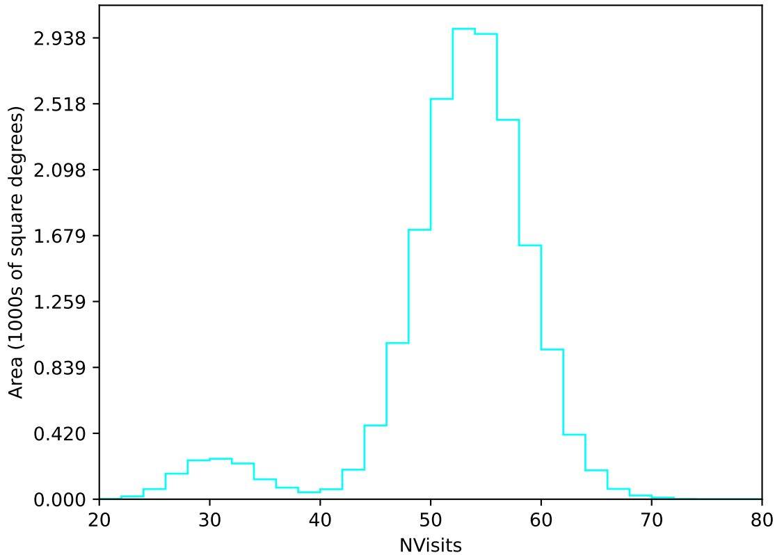
roll_uniform_early_half_accordion1_mjdp0_v3.4_10yrs WFD u band: NVisits
