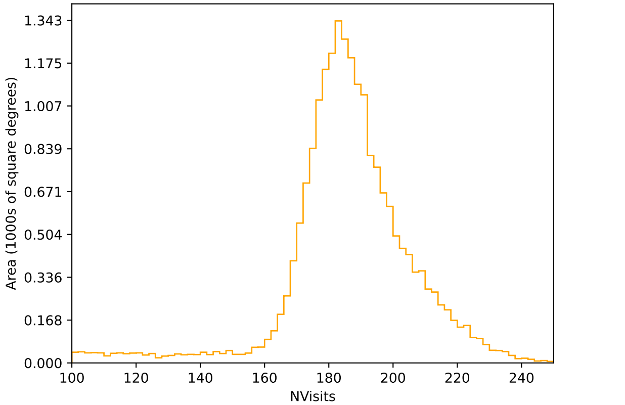
roll_uniform_early_half_accordion1_mjdp0_v3.4_10yrs All sky r band: NVisits
