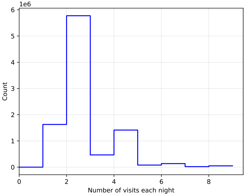
roll_uniform_early_half_accordion1_mjdp0_v3.4_10yrs All sky: NVisitsPerNight
