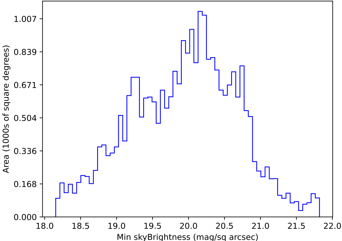
roll_uniform_early_half_accordion1_mjdp0_v3.4_10yrs All sky g band: Min skyBrightness
