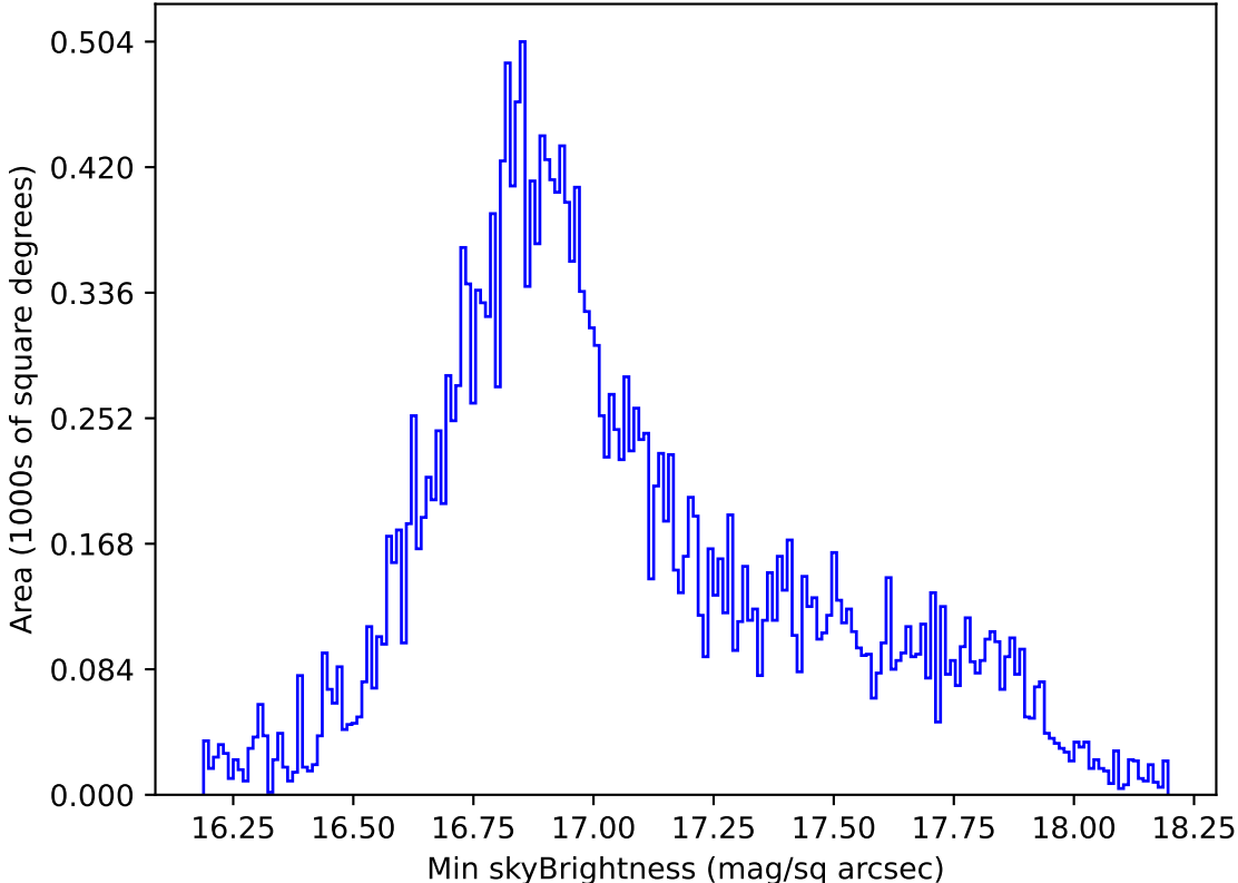
roll_uniform_early_half_accordion1_mjdp0_v3.4_10yrs All sky all bands: Min skyBrightness
