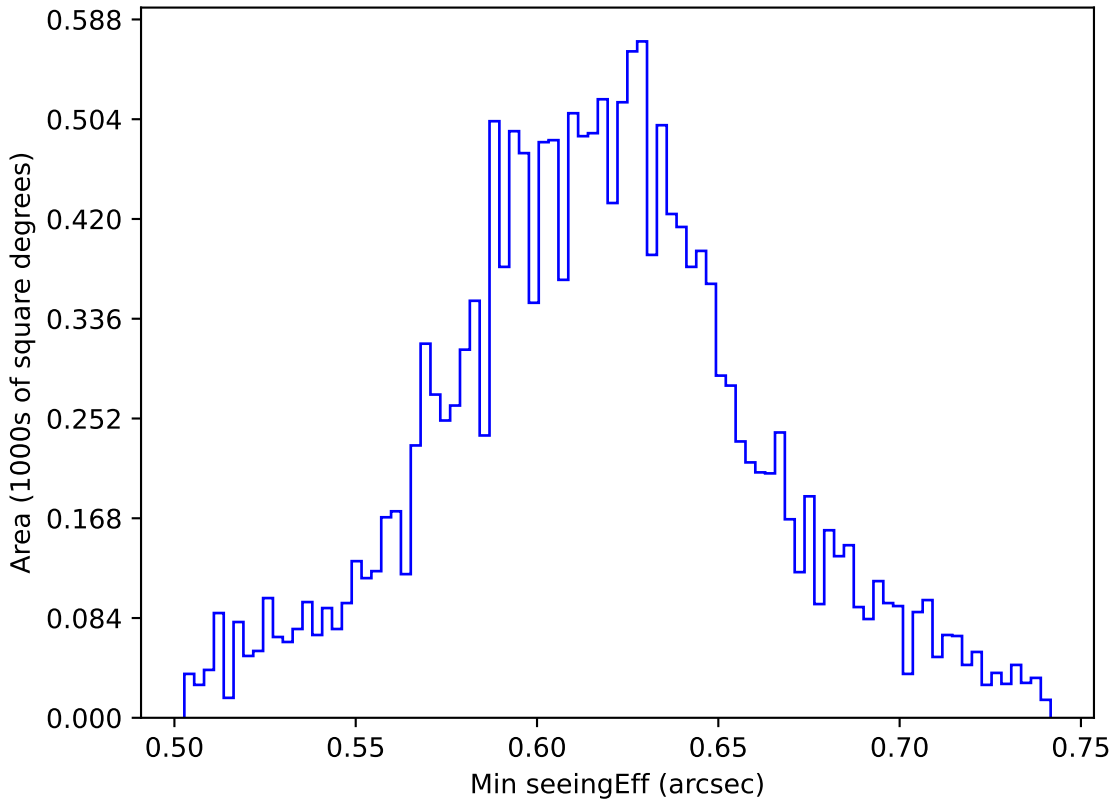
roll_uniform_early_half_accordion1_mjdp0_v3.4_10yrs WFD z band: Min seeingEff
