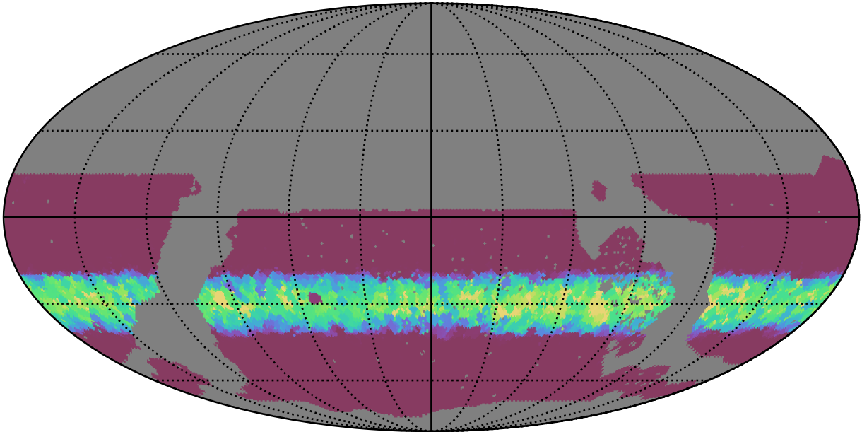
roll_uniform_early_half_accordion1_mjdp0_v3.4_10yrs WFD z band: Min normairmass
