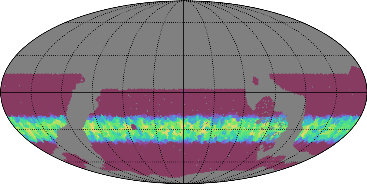
roll_uniform_early_half_accordion1_mjdp0_v3.4_10yrs WFD g band: Min normairmass
