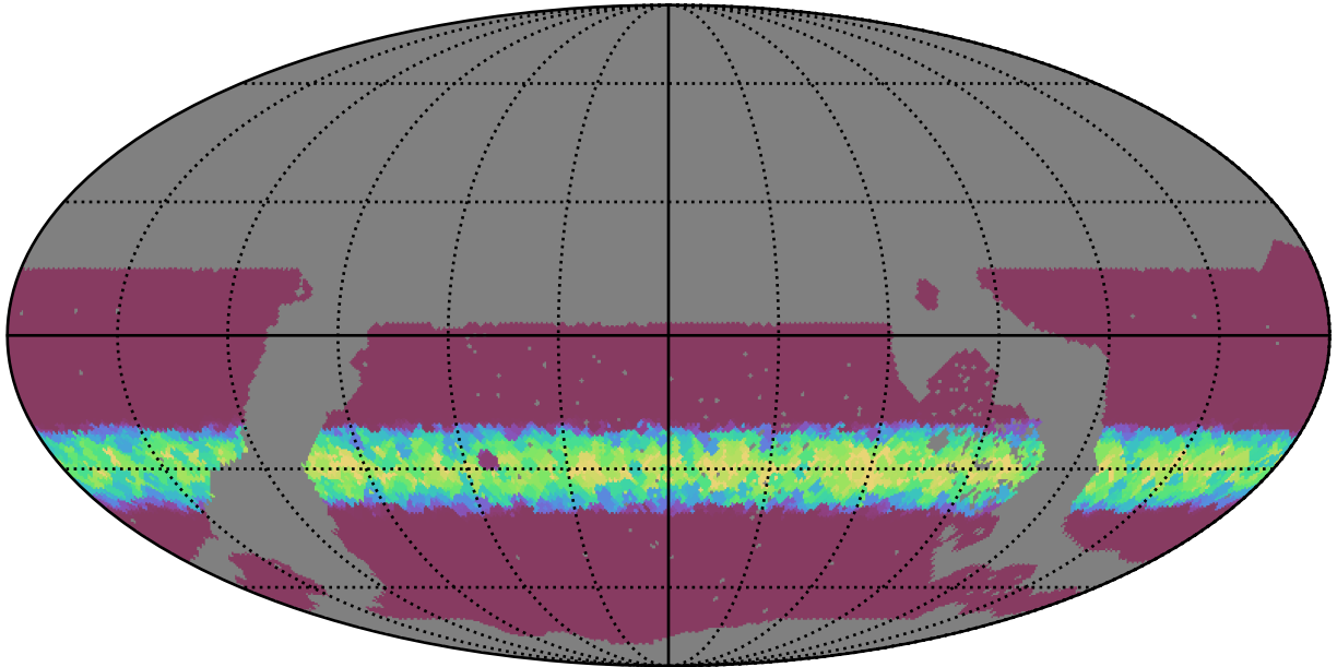
roll_uniform_early_half_accordion1_mjdp0_v3.4_10yrs WFD all bands: Min normairmass
