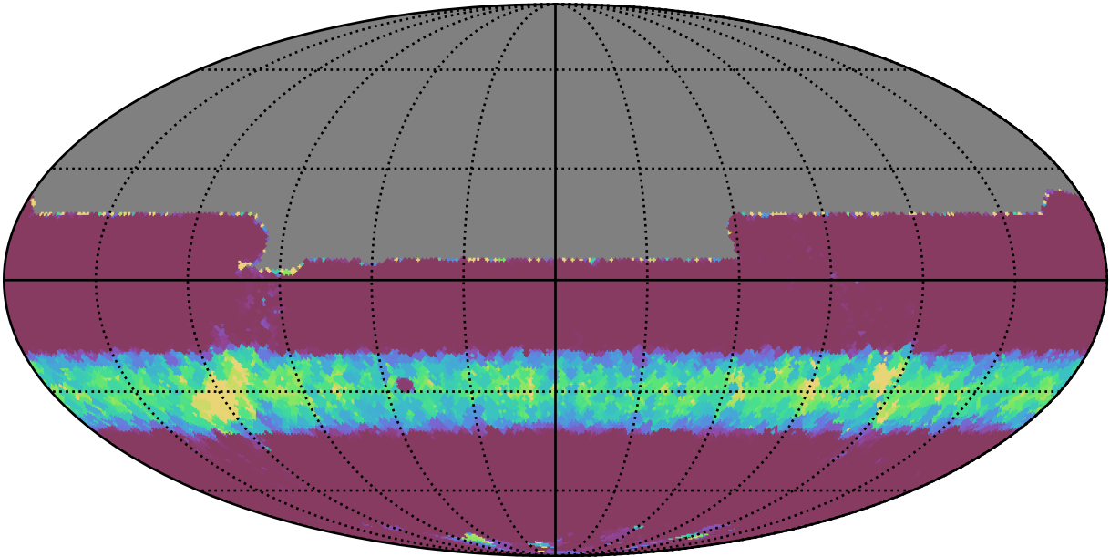
roll_uniform_early_half_accordion1_mjdp0_v3.4_10yrs All sky y band: Min normairmass
