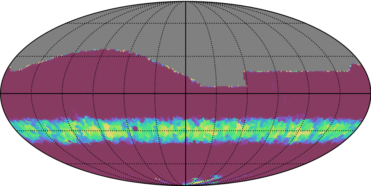
roll_uniform_early_half_accordion1_mjdp0_v3.4_10yrs All sky r band: Min normairmass
